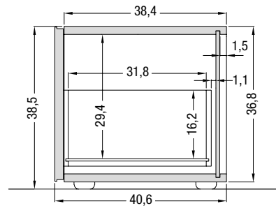
1 cestone 1 deep drawer
