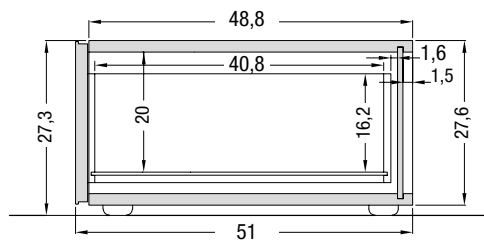
1 cestone 1 deep drawer
