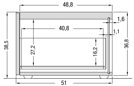
1 cestone 1 deep drawer
