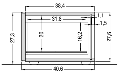
1 cestone 1 deep drawer
