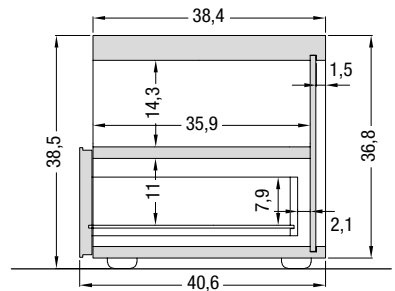
1 cassetto + vano a giorno 1 drawer + open compartment
